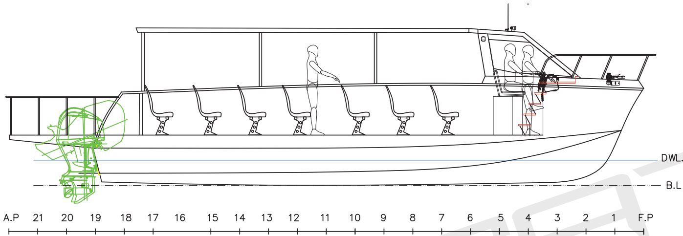
STBD SIDE PROFILE
